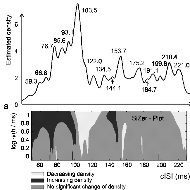
Figure 3. a. Kernel density estimate of all cISI and modal values. b. Result of an analysis with SiZer.
